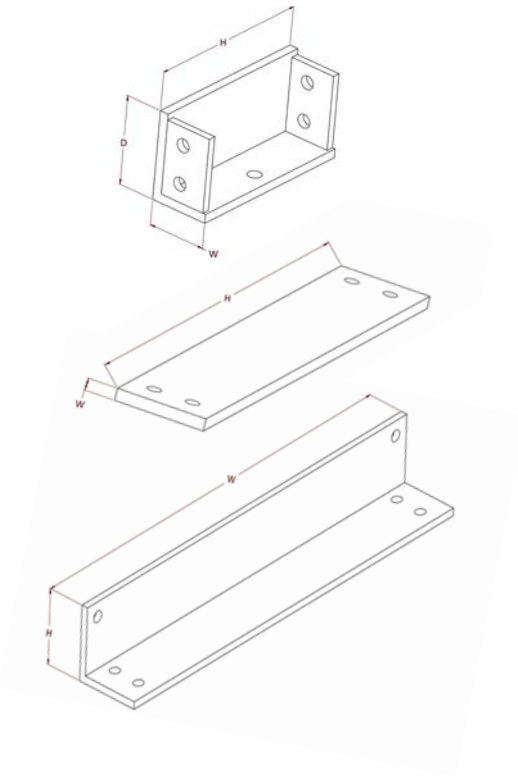
WallMax® Modular Frame (WMF)
