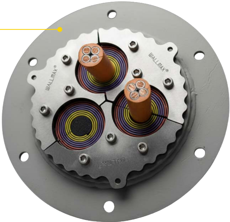
WallMax® Round Dynamic (WRD)
